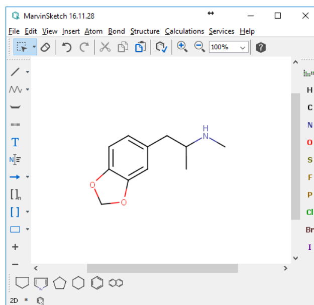
Figure 8. MarvinSketch used to draw 2D molecular structure
