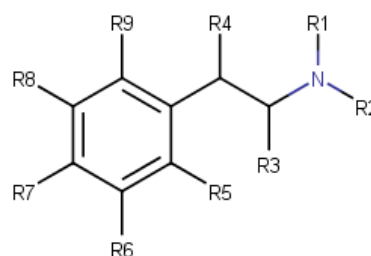
Figure 3. Basic 2D molecular structure of ATS [2]
