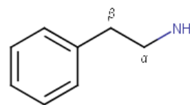
Figure 2. 2D molecular structure of \beta -phenethylamine [2]
