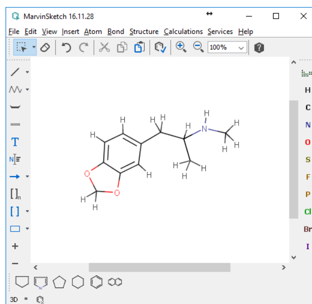
Figure 9. MarvinSketch used for 3D conversion
