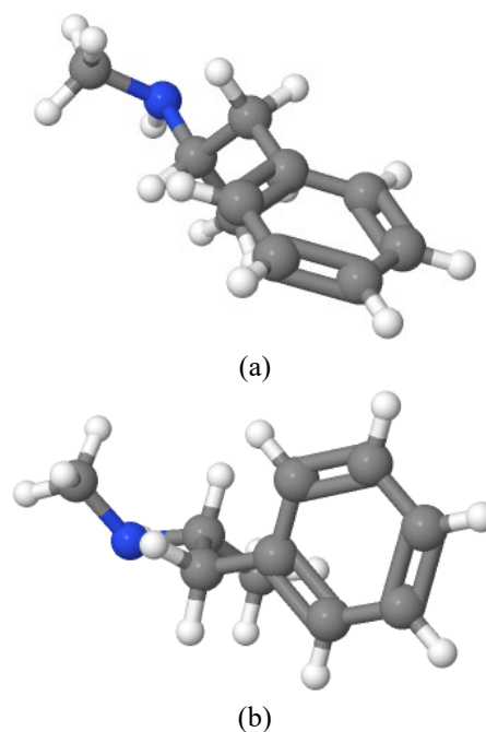
Figure 7. 3D molecular structure of (a) d -methamphetamine and (b) l -methamphetamine
