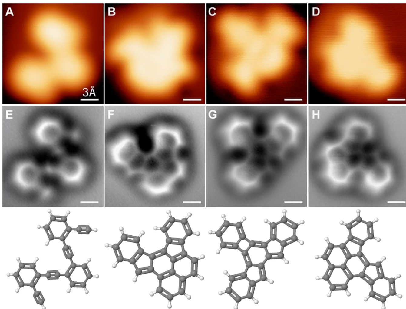
Figure 1. Comparison of STM images, nc-AFM images, and 3D molecular structures model [30]
