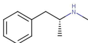
Figure 6. 2D molecular structures of l -methamphetamine [48]
