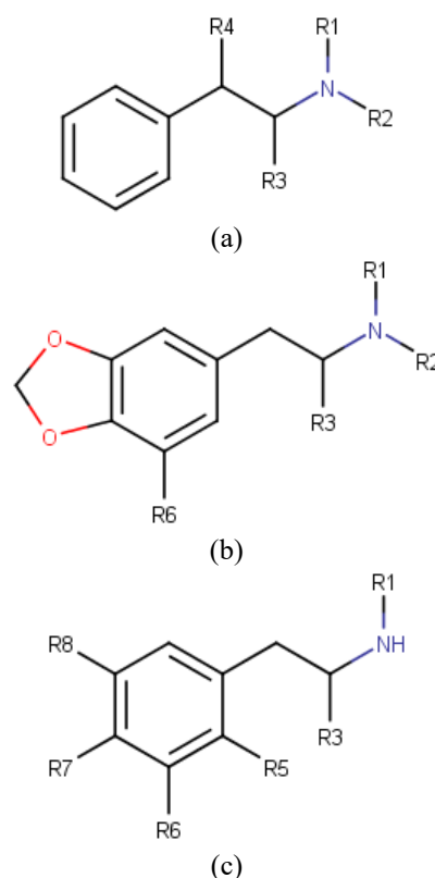
Figure 4. Sub-groups of ATS per substitution patterns: (a) no substitution, (b) methylenedioxy-substitution, and (c) other substitution patterns [2]
