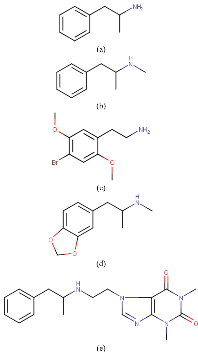
Figure 5. Samples of ATS drug molecular structure: (a) amphetamine, (b) methamphetamine, (c) 2C-B, (d) MDMA, and (e) fenethylamine [2]
