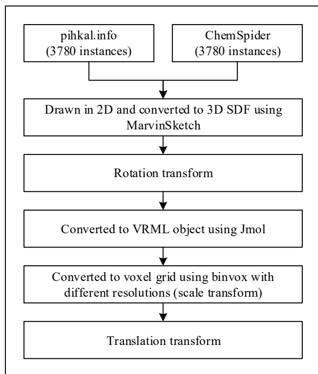
Figure 15. Summary of dataset preparation process
